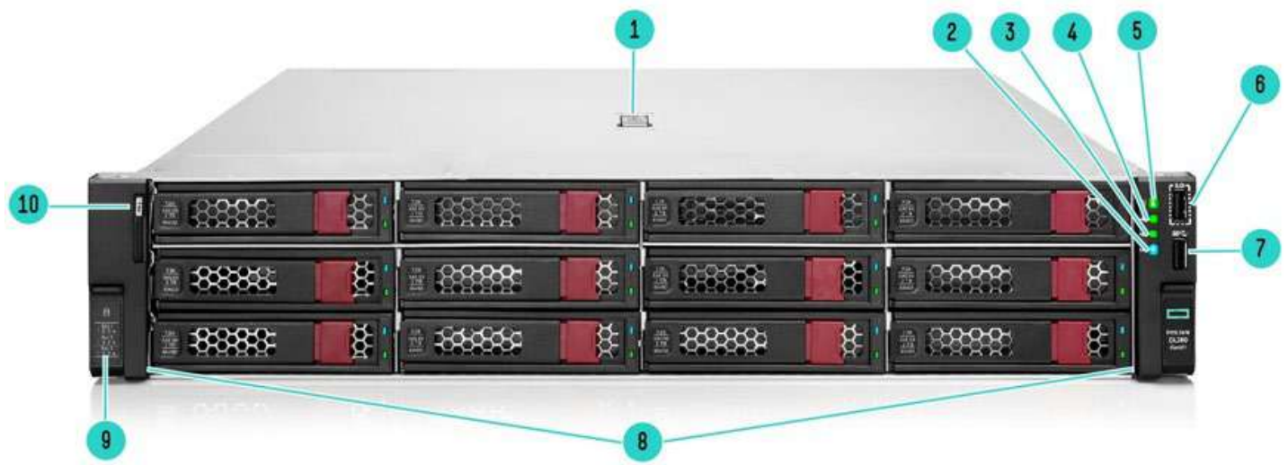
Front View – 12LFF chassis shown
