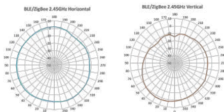
BLE/ZigBee 2.4GHz plots
